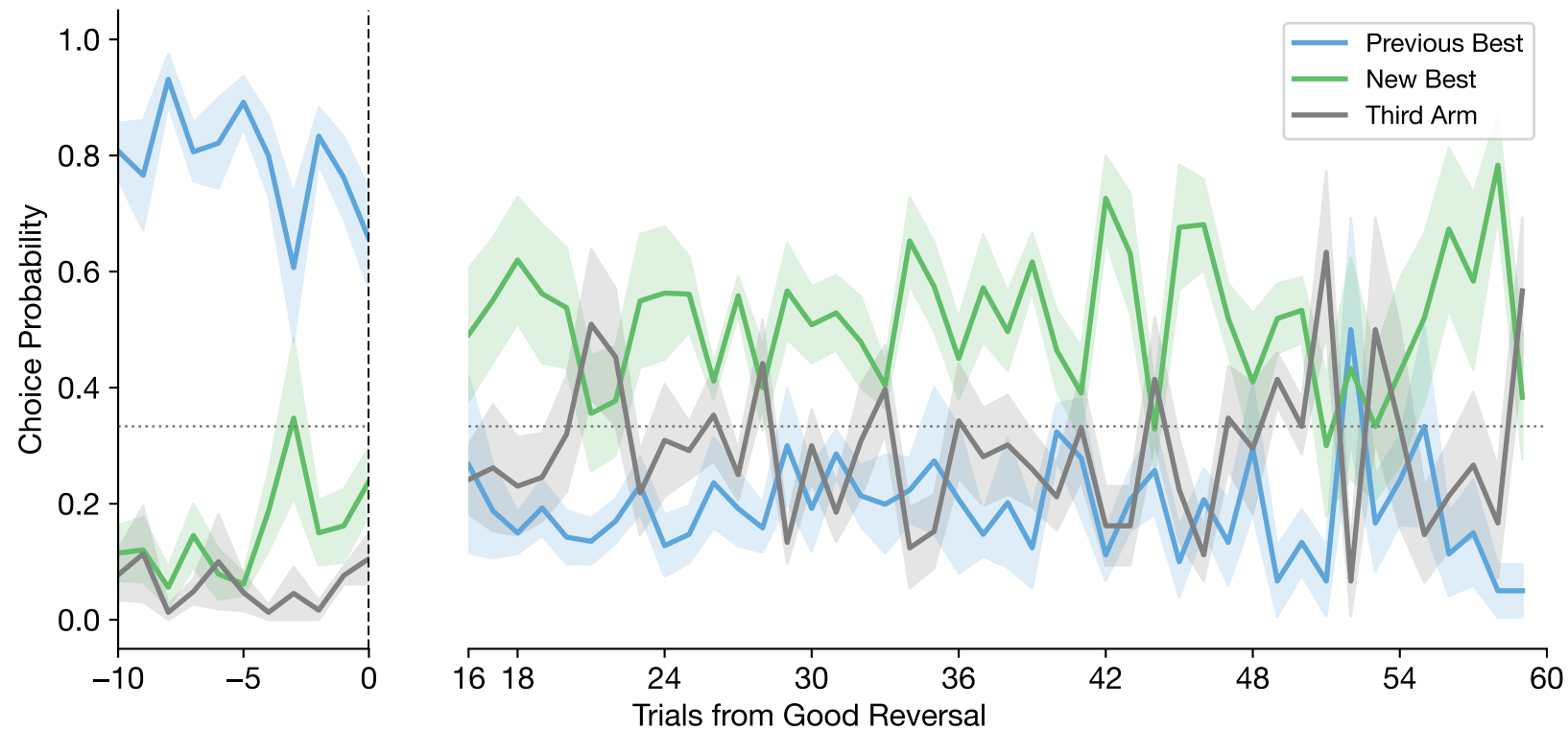
Good Reversal-Aligned Choices (mean \pm se across subjects | n=6 subjects, n=57 reversals) (Skipping first 15 trials post-reversal)
